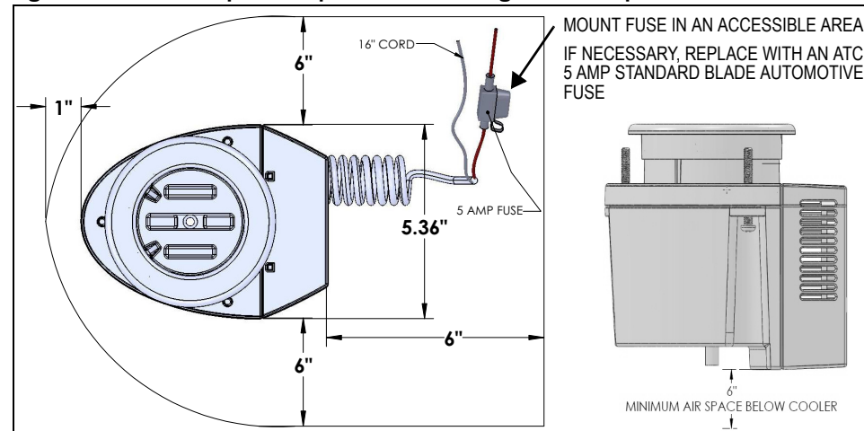
Figure 1: Ventilation Space Required for Mounting Eskimo Cup
