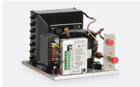
ADLER/BARBOUR COLDMACHINE KIT CU-100 & VD-150
